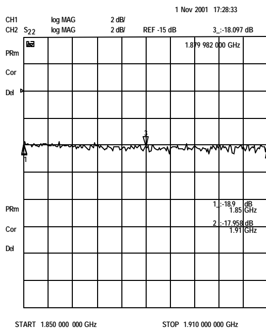
Output Return Loss at 25 °C
