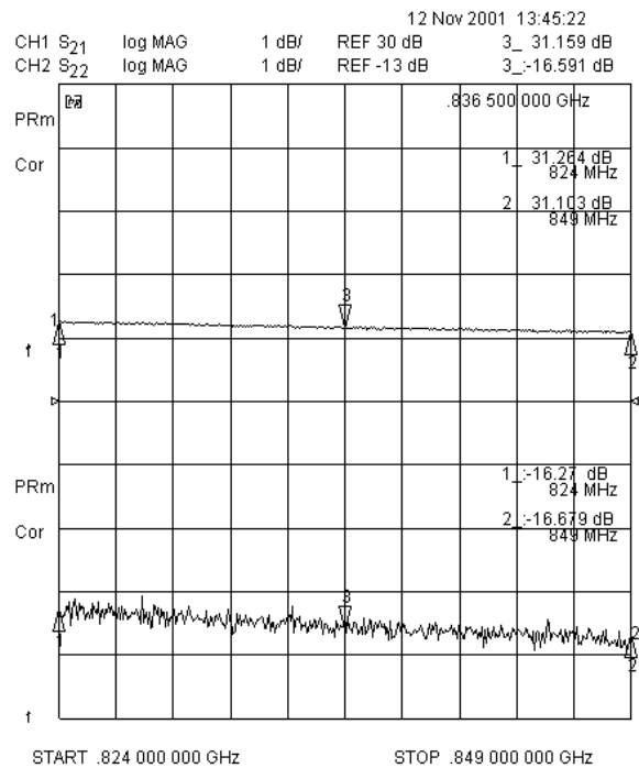
Gain and Output Return Losses at 25 °C
